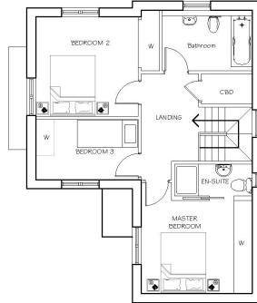
FIRST FLOOR PLAN PLOT 26
